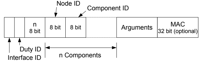
Figure 3. SpartanRPC data packet format.
